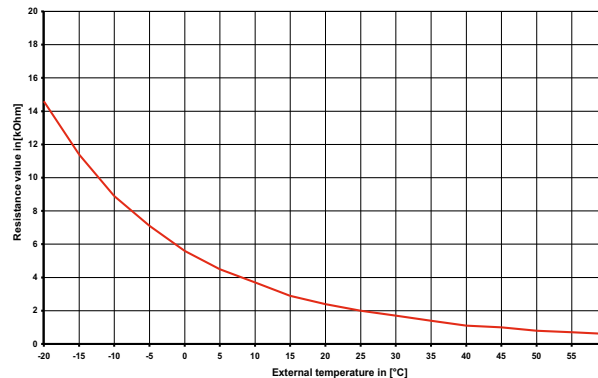
Fig. 7.2: Sensor characteristic curve NTC-2 according to DIN 44574 Outside temperature sensor
